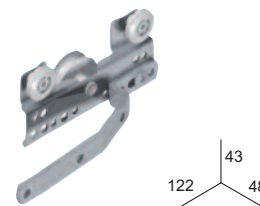
CORREDERA MAESTRA
