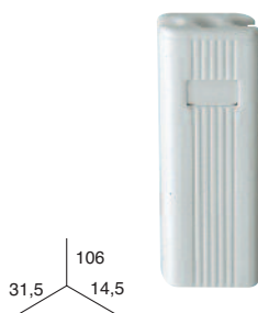
CONTRAPESO 70 grs.
