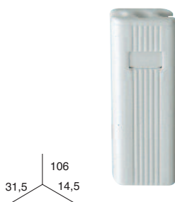
CONTRAPESO 110 grs.
